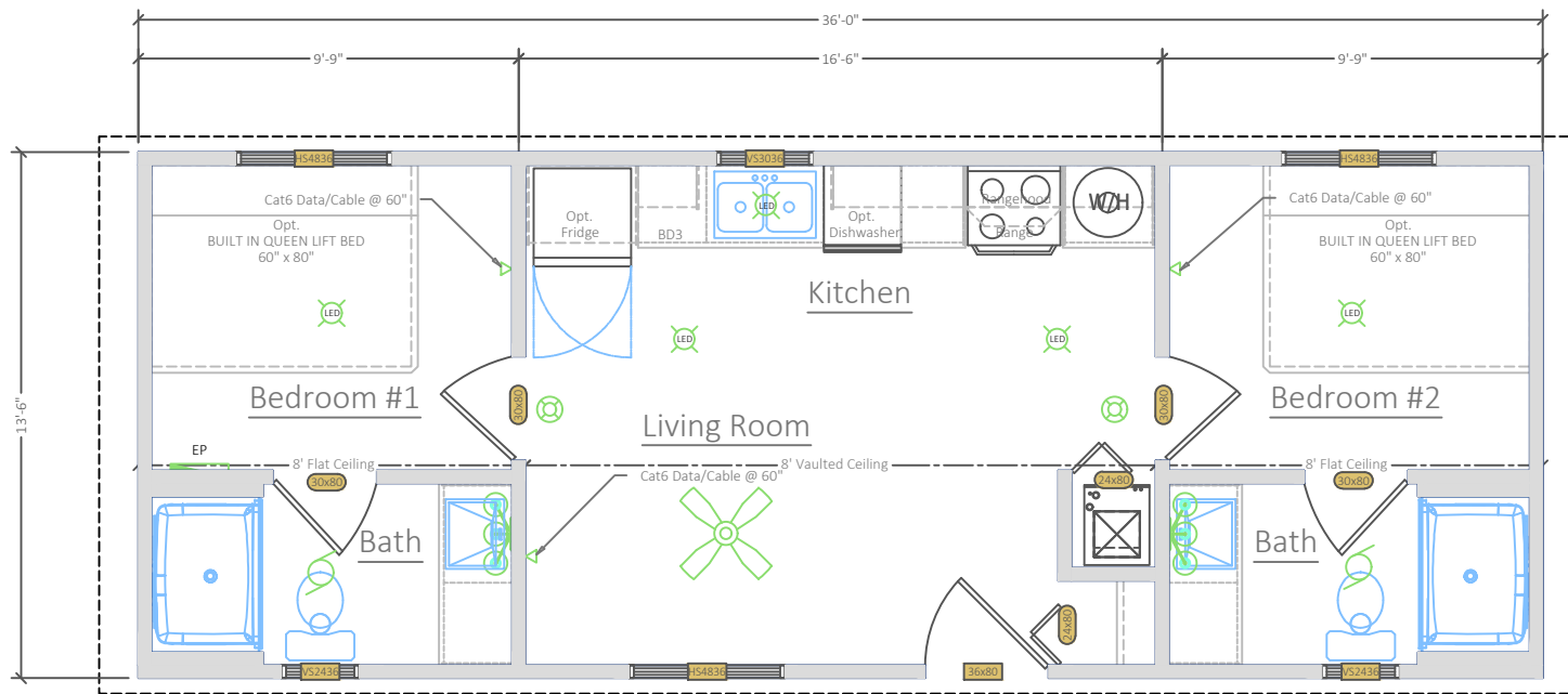
1 Main Floor Plan A1 SCALE: 1/4" = 1'-0"
