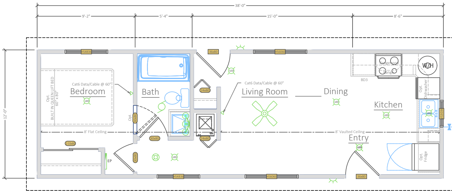
1 Main Floor Plan A1 SCALE: 1/4" = 1'-0"
